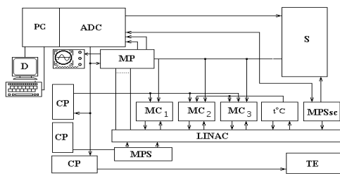
Fig. 1. Functional layout of the EPOS linac control system
