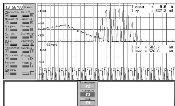
Fig. 3. Videogram of the total beam profile monitor signal measurement (pulse train at the top of videogram).
