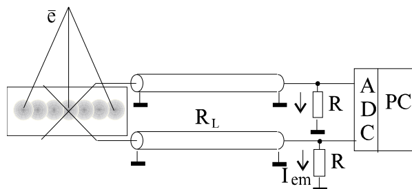
Fig. 7. Structure schematic for two-dimension beam
