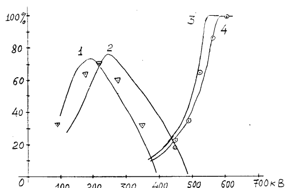
Fig. 3. Dependence of the AT calculated currents on the AT voltage.
