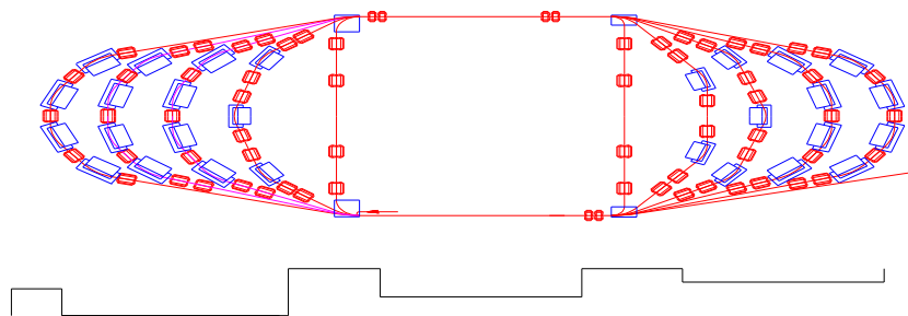
Fig. 1. Recirculator lay-out in variant 1
