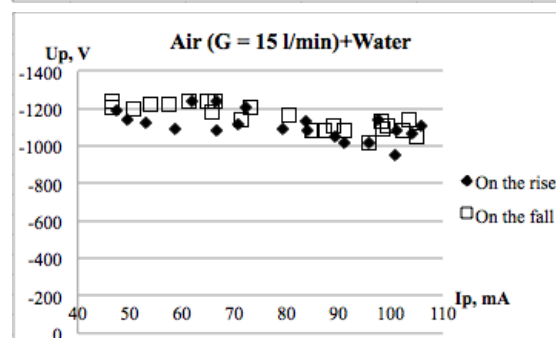
Fig. 9. Volt-ampere characteristics of the primary discharge for different plasma-forming gas flow rates determined from oscillograms
