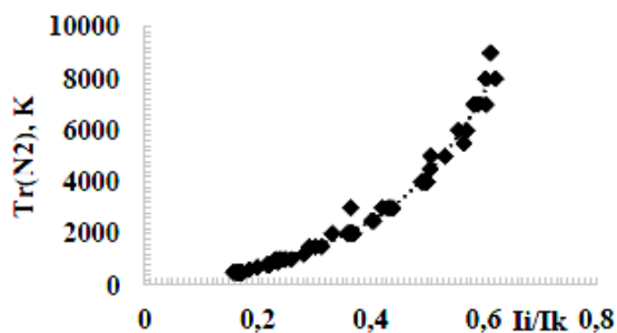
Fig. 5. Dependence of the temperature of the N 2 rotational levels population on the ratio of intensities in the band (0-0) of the 2+ system at \lambda_i = 335.9 , \lambda_k = 336.9 nm
