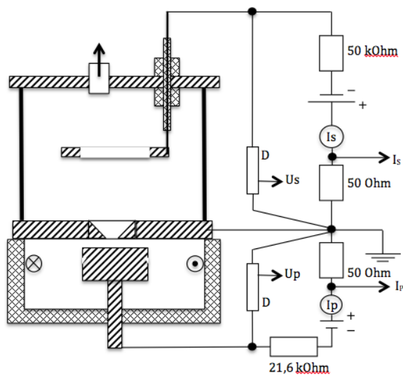
Fig. 2. Discharge powering scheme
