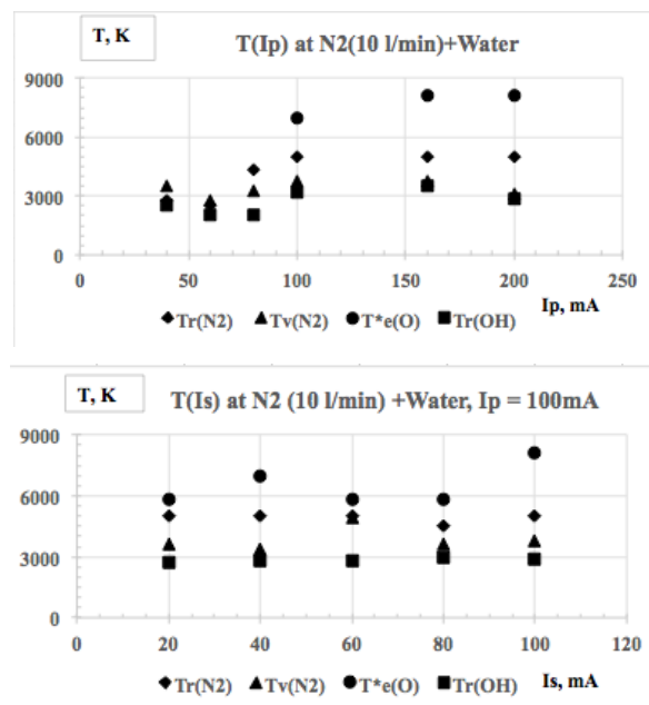
Fig. 16. Dependence of the temperatures of the population of O I electron levels, N_2 vibrational levels and N_2 and OH rotational levels on discharge currents
