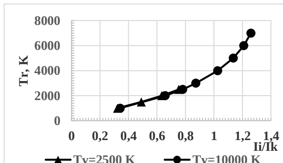
Fig. 4. Dependence of the temperature of the OH rotational levels population on the ratio of intensities in the band (A-X) at \lambda_i = 306.7 , \lambda_k = 308.9 nm
