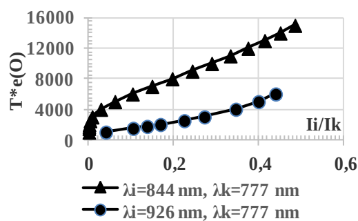
Fig. 3. Dependence of the temperature of the O I electron levels population on the ratio of intensities of inseparable multiplets with \lambda = 777, 844, 926 nm
