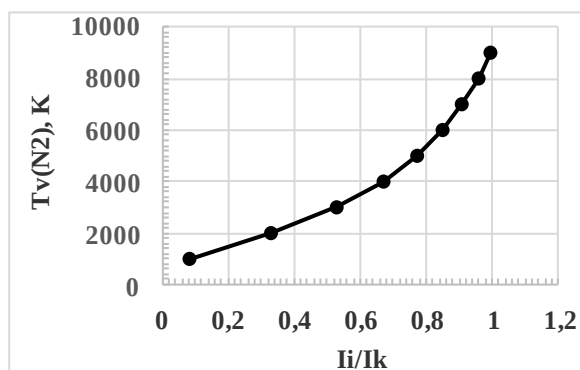
Fig. 6. Dependence of the temperature of the N 2 vibrational levels population on the ratio of intensities in the 2+ band system at \lambda_i = 315 , \lambda_k = 337 nm
