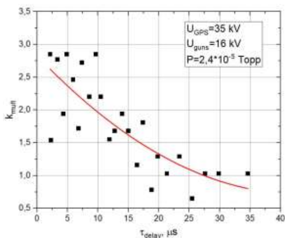
Fig. 14. The effect of delay time on the value of the multiplication factor
