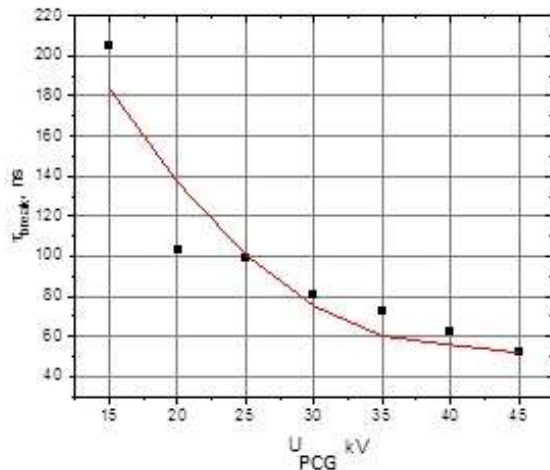
Fig. 8. Dependence of the POS opening time on the main circuit voltage
