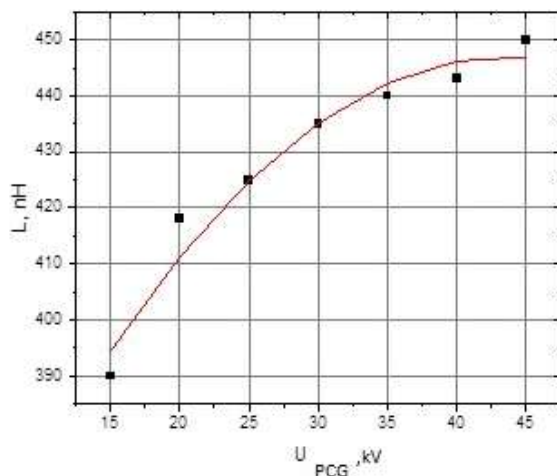
Fig. 9. Inductance of the main circuit during energy storage mode depending on the main circuit voltage
