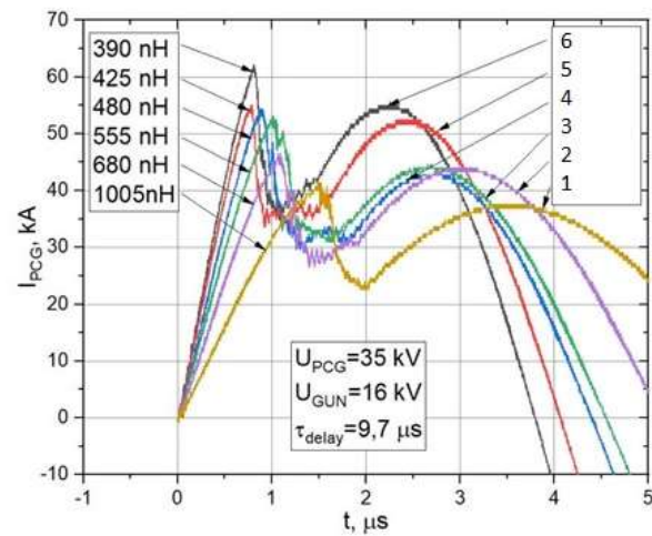
Fig. 10. The effect of inductance on the current value of the main circuit and the angle of the curve during POS operation
