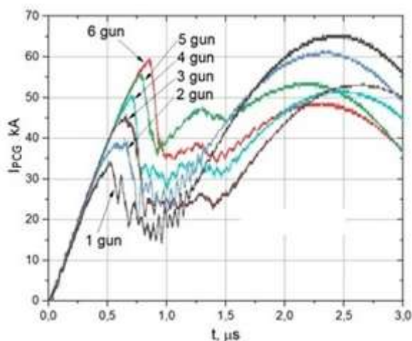
Fig. 13. Time dependence of the main circuit current for different plasma guns' number used to power the POS
