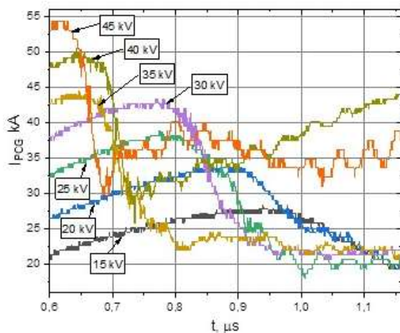
Fig. 4. Time dependence of the main circuit current for the current interruption time for different PCG voltages
