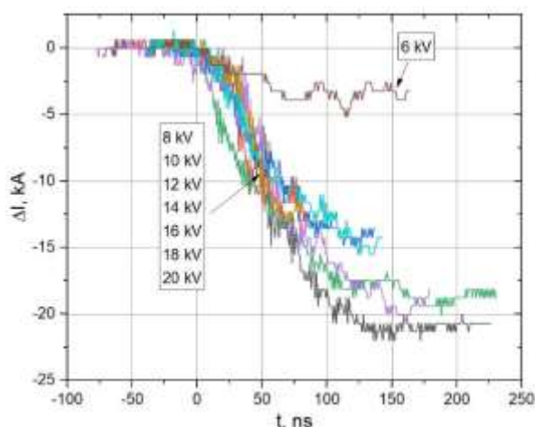
Fig. 12. Change rate of the POS current (in time of current interruption) for different plasma gun voltages
