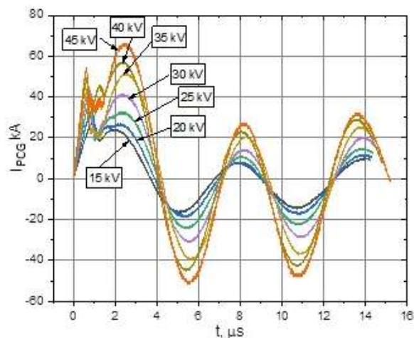
Fig. 3. Time dependence of the main circuit current for different PCG voltages
