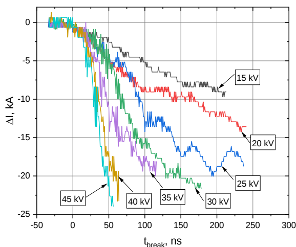
Fig. 5. Change rate of the POS current (in time of current interruption) for different PCG voltages
