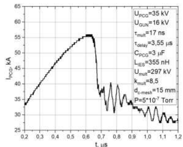
Fig. 6. Oscillograms of the main circuit current with the POS tripping
