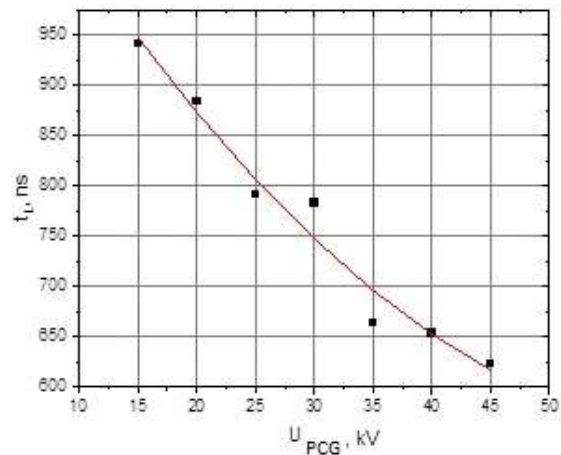
Fig. 11. Dependence of energy accumulation time on the charging voltage of the main circuit
