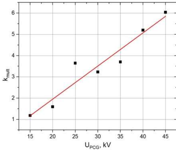
Fig. 7. Dependence of the multiplication factor on the main circuit voltage
