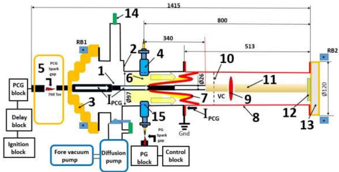
Fig. 1. DIN-2K electron accelerator schematic diagram. 1 is the tubular cathode; 2 is the grounded accelerator chamber body, anode; 3 is the vacuum insulator; 4 is plasma guns; 5 is the air gap; 6 is the POS; 7 is the S-shaped plasma current density in the POS [13–15]; 8 is the waveguide; 9 is the virtual cathode (VC); 10 is the anode mesh; 11 is the electron beam; 12 is the quartz protective glass; 13 is the plexiglass end flange; 14 is the vacuum tube; 15 is plasma guns; PCG is the pulse current generator; RB1, RB3 are Rogovsky belts
