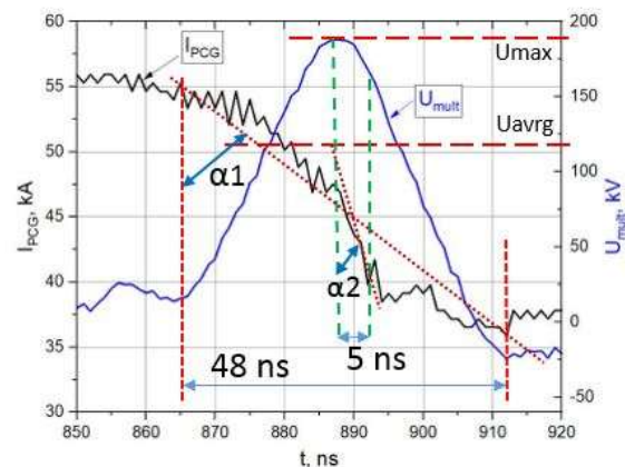
Fig. 2. The main circuit current dynamics in the POS operation time (current interruption time) and the calculated shape of the induced voltage curve
