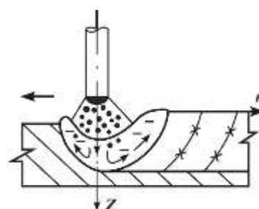
Fig. 3. Scheme of approximation of the longitudinal section of the weld pool
