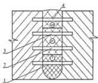
Fig. 7. Diagram of the samples 1–4 cut out from the welded joint to study the output structure. I–III – joint sections: I – lower, II – middle, III – upper
