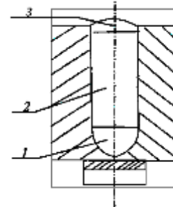
Fig. 5. Cross-sectional diagram of the rotor welded joint of the pilot model:
