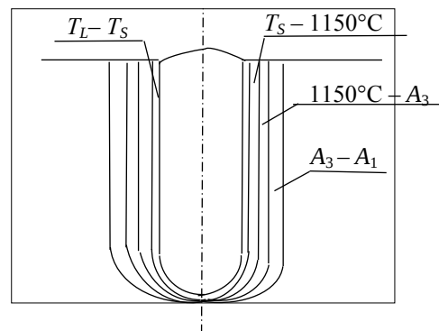
Fig. 6. Temperature fields obtained by modelling of the temperature regime of the rotor welded joint
