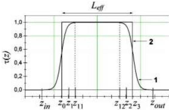
Fig. 2. Representation of the longitudinal distribution profile of the quadrupole field component: 1 – real field distribution; 2 – approximation of the field distribution with reduction to the effective length (rectangular model)
