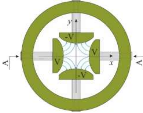
Fig. 1. Schematic representation of an electrostatic quadrupole lens
