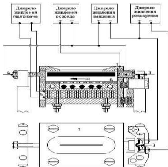
Ion source design: 1 – anode; 2 – heated cathode; 3 – cathode filament; 4 – anticathode; 5 – FCP ceramic heater; 6 – replaceable insert
