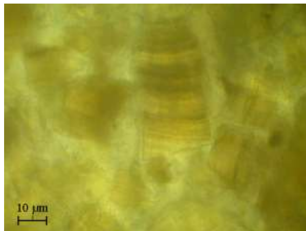
Fig. 4. Microphotograph of a kidney stone from 2024 year, consisting of whewellite (calcium oxalate monohydrate). Under transmitted light without an analyzer
