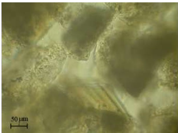
Fig. 3. Microphotograph of a kidney stone from 2019 year, consisting of large apatite (calcium phosphate) grains and whewellite (calcium oxalate monohydrate). Under transmitted light without an analyzer
