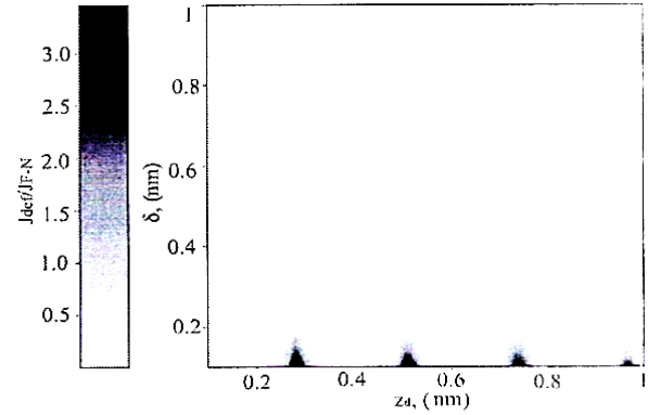
Fig. 2. The ratio of the emission current density from the modified surface j_{def} to the Fowler-Nordheim current j_{F-N} depending on the layer thickness \delta and the depth z_d [7]
