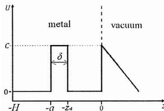
Fig. 1. Schematic representation of the model of a near-surface layer with radiation defects in form of a rectangular potential barrier [7, 9, 10]
